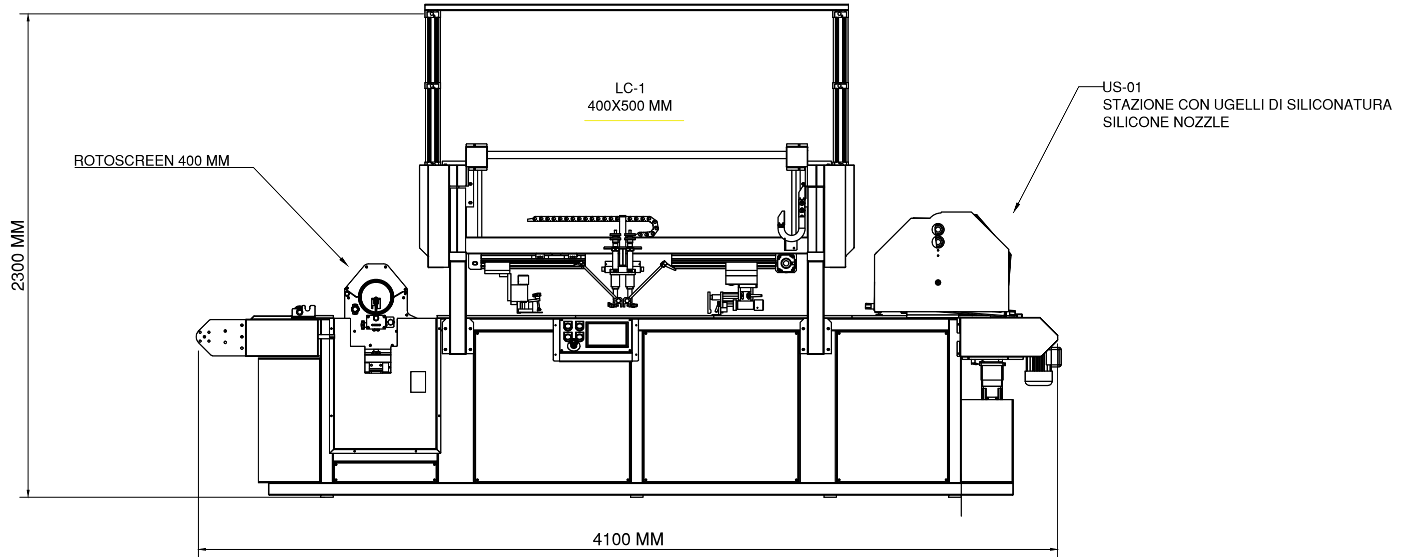
ROTOSCREEN 400 + LC-01 400X500 MM + US-01
